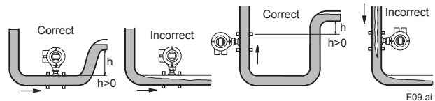
Mounting Positions
